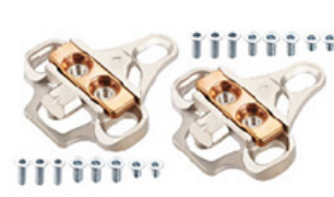
RC8 (126 g/pr) New cleat design for mountain clipless pedal to be assembled on LOOK style shoes. MATERIAL : Cr-Mo
